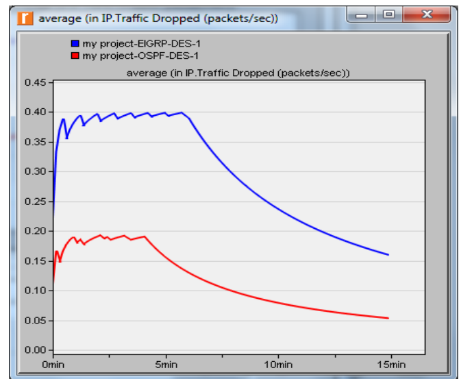
Fig 4.3 Traffic dropped (packets/sec) in case of situation 1
