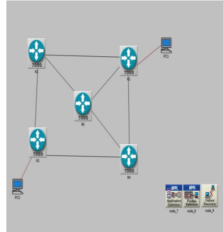
Fig 3.1 OPNET simulated network topology.
